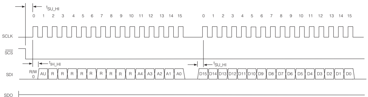
Figure 3-6: Write Cycle
