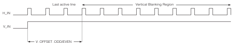
Figure 3-2: Vertical Offset Definition
